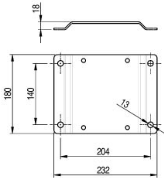
FIXING BRACKET
